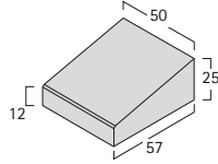
central v57vg v57vg central 115Kg 50 L x 57 P(D) x 25 H cm
